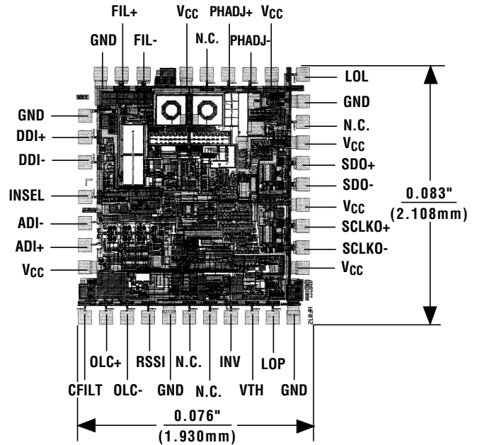
Chip Topography
